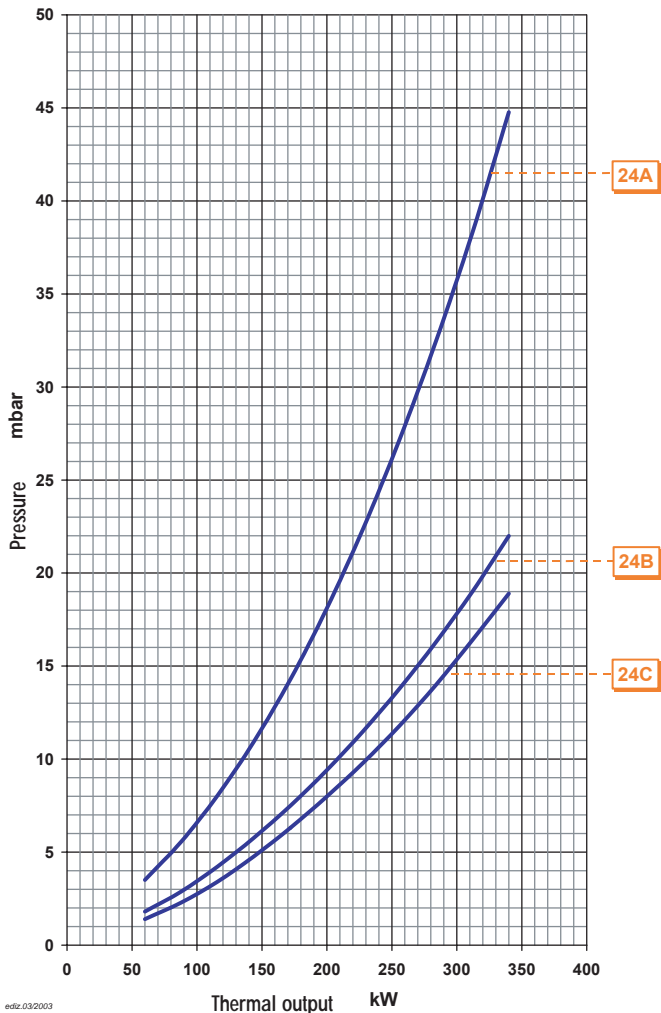
Head loss (combustion head + gas train + pressure regulator) BGS 30LX Natural gas CE / EXP
